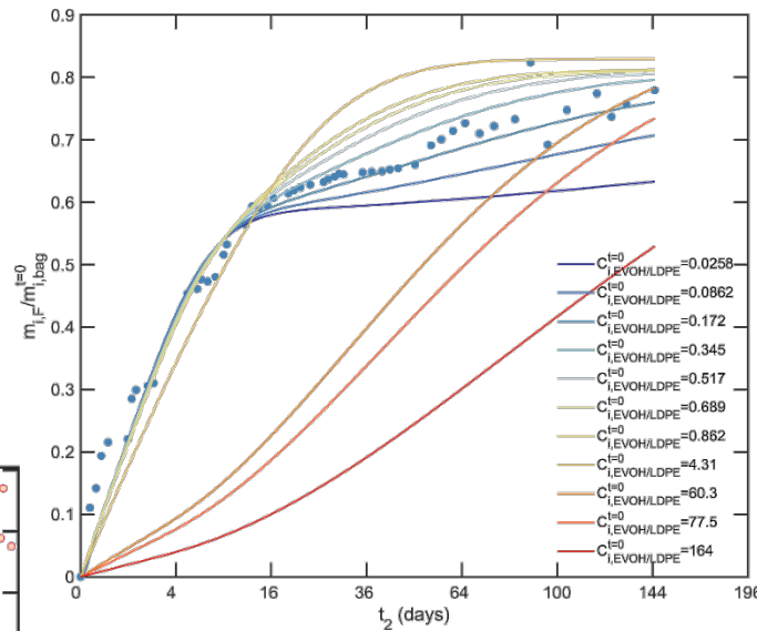
Effect of initial distribution of migrant in multilayer packaging on migration kinetic of Irganox 1010 into ethanol
