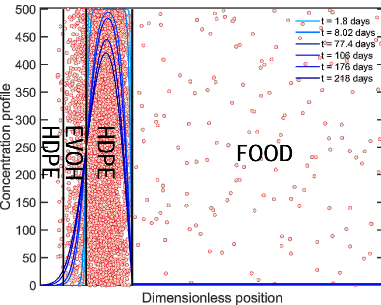
Concentration profiles of Irganox 1076 in a trilayer packaging of 400 \mu\text{m} of thickness in contact with milk at 25°C
